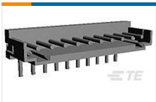
TE Part #292253-2 CT CONN MT HDR ASSY H 2P NAT
