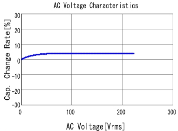
■ GRM31A7U2J101JW31 C-AC Voltage capchange, DC0V, 25.0d
