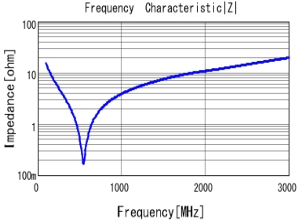
■ GRM31A7U2J101JW31 |Z| DC0V, 25degC
