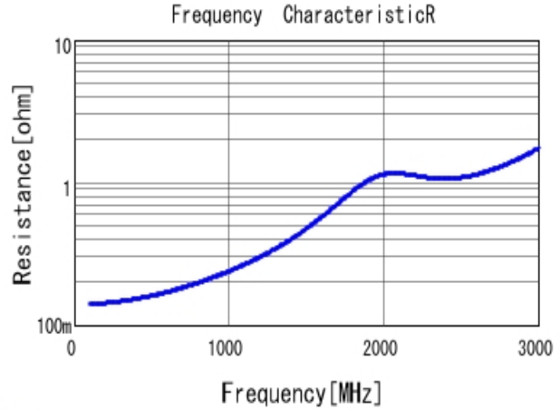
■ GRM31A7U2J101JW31 R DC0V, 25degC
