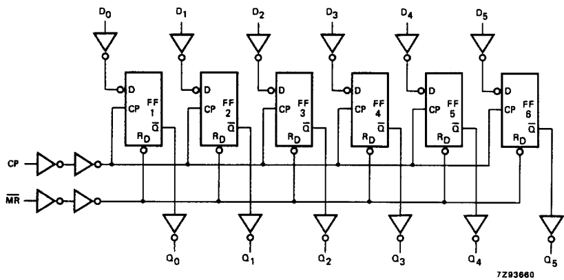
Fig.5 Logic diagram.
