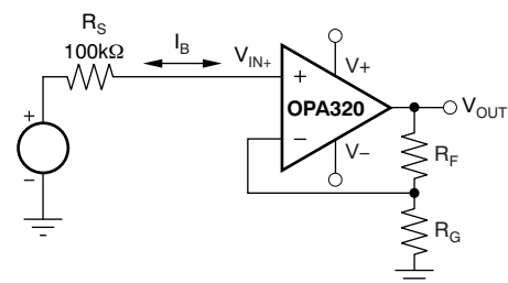
Figure 42. Noise as a Result of I_{BIAS}
