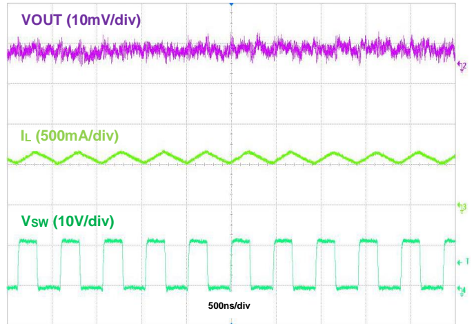
Figure 15. Output Voltage Ripple, V OUT = 5V; IOU = 600mA
