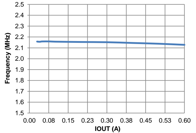
Figure 13. f sw vs. IOU (A)
