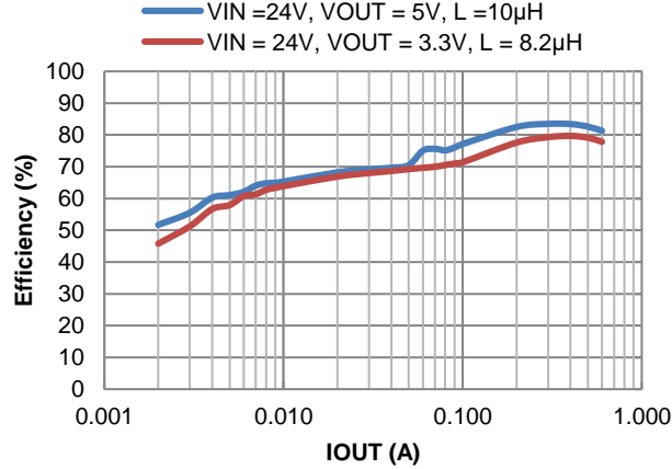
Figure 5. Efficiency vs. Output Current, V_{IN} = 24\text{V}
