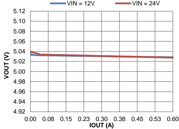
Figure 7. Load Regulation
