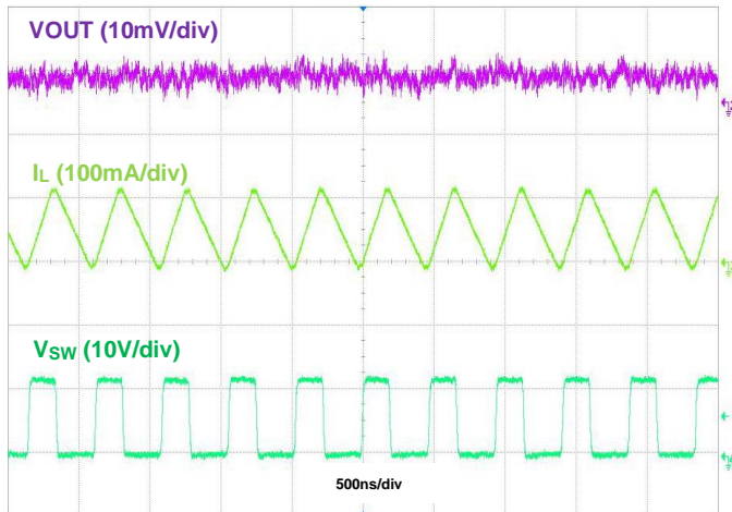
Figure 14. Output Voltage Ripple, V OUT = 5V; IOU = 50mA
