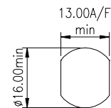
PANEL PIERCING DETAILS
