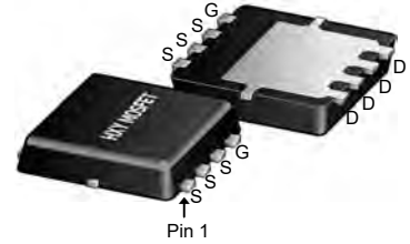
DFN5X6-8L (DFN-8-EP(6.1x5.2))
