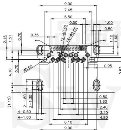
RECOMMENDED PCB LAYOUT PCB T=1.20mm TOL:±0.05
