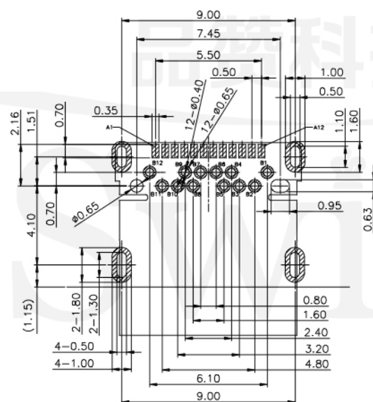
RECOMENDED PCB LAYOUT PCB T=1.20mm TOL:±0.05
