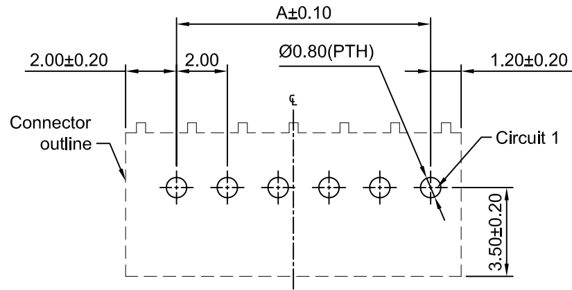
P.C.B LAYOUT TOLERANCE:±0.05
