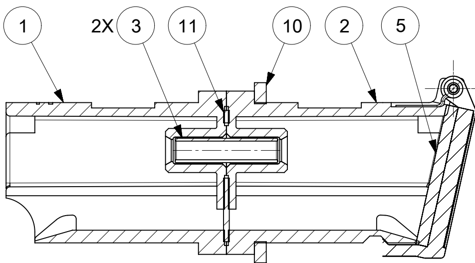
SECTION Z-Z
