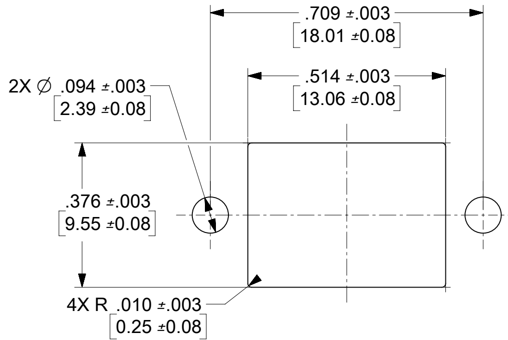
RECOMMENDED MOUNTING PATTERN
