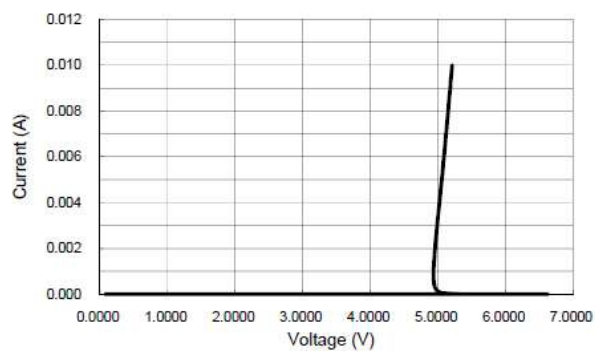
Fig 3 Voltage Sweeping
