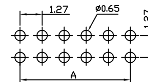
RECOMMEND P.C.B LAYOUT PCB TOLERANCE: ±0.05 (TOP VIEW)
