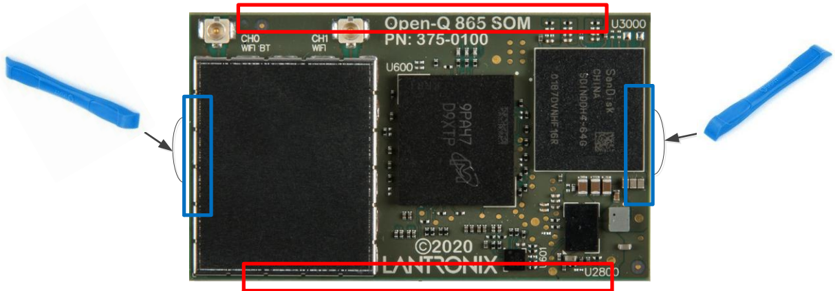
Figure 12. SOM Plastic Prying Tool Removal Locations
