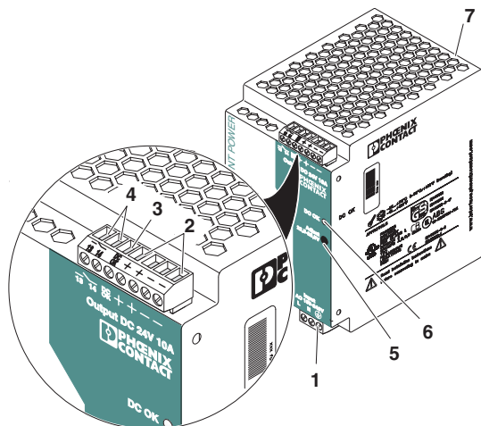
Figure 1 Operating elements
