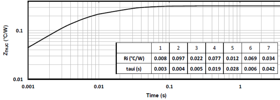
Figure 18 • Maximum Thermal Impedance
