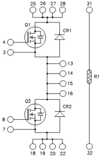
Figure 1 • MSCSM70AM07CT3AG Electric Schematic
