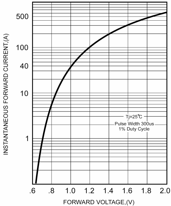
FIG.1-TYPICAL FORWARD CHARACTERISTICS
