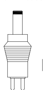
Hohlstecker/ hollowplug 1,7x4x10mm Art.Nr.:10950399/01
