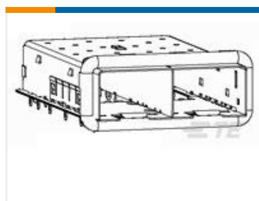
TE Part #2198720-1 zSFP+ 1x2 Cage Assembly, Press-Fit
