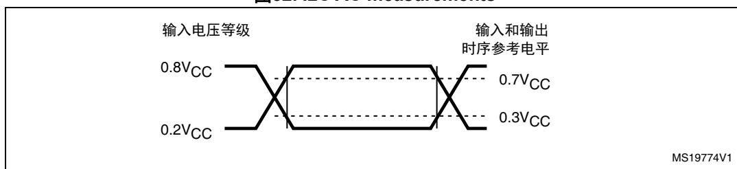
图32. I2C AC measurements
