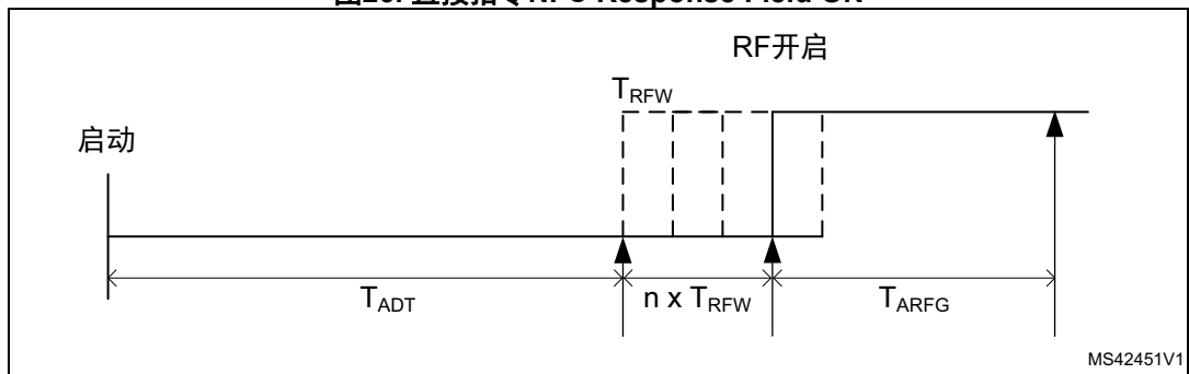
图26. 直接指令NFC Response Field ON
