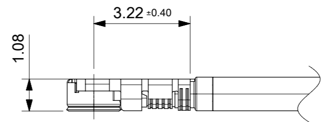
MHF4 CONNECTOR
