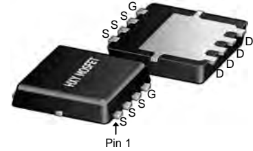
DFN5X6-8L (TDSO8-EP(5.1x5.9))
