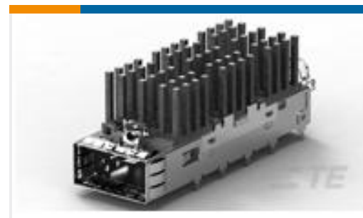
TE Part #1888971-3 QSFP TB Cage Assy, w/LP, PCI HS
