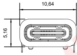
Sketch with waterproof ring
