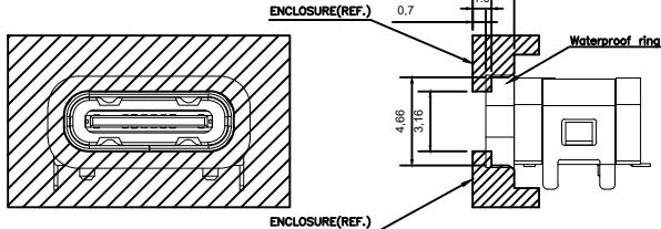
RECOMMENDED SCHEMATIC DRAWING OF CONNECTOR MATCH CHASSIS
