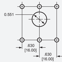
Three Pole
