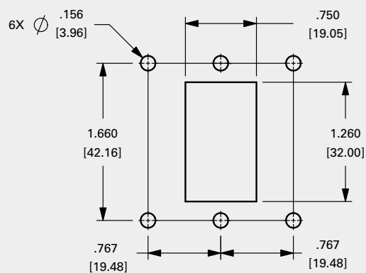
THREE POLE
