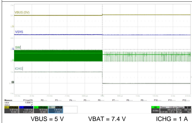
Figure 72. Charge Disabled
