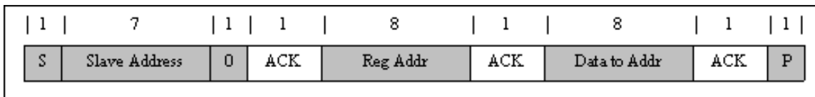
Figure 19. Single Write
