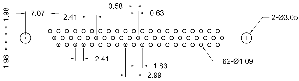
Recommended PCB Layout (Top View)
