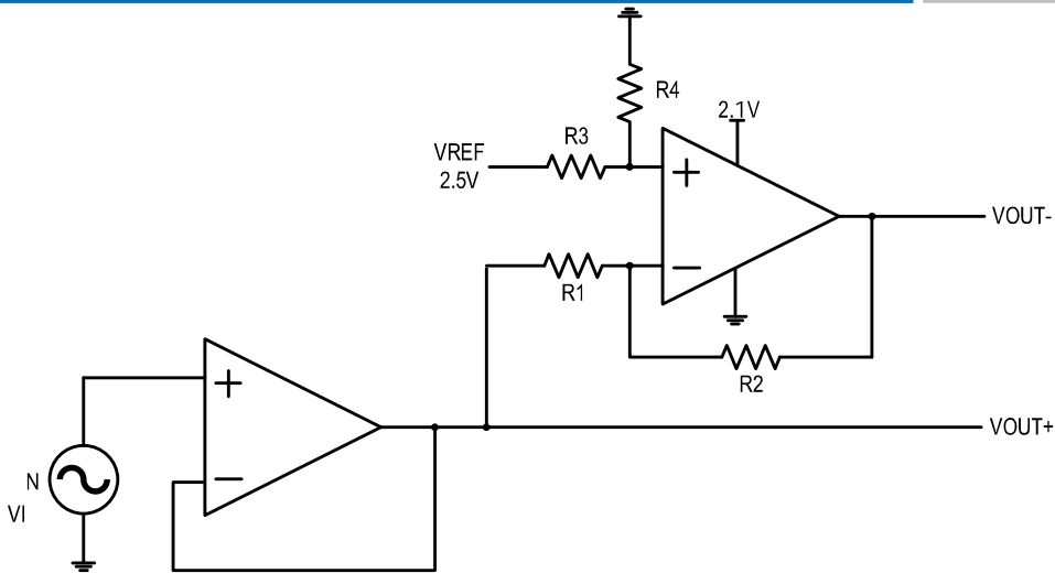
Figure 13. Schematic for Single-Ended Input to Differential Output Conversion
