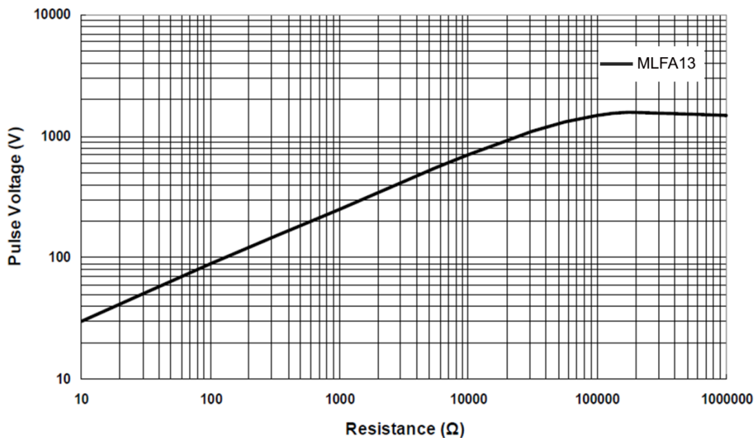
MLFA13 10/700µs Lightning Surge
