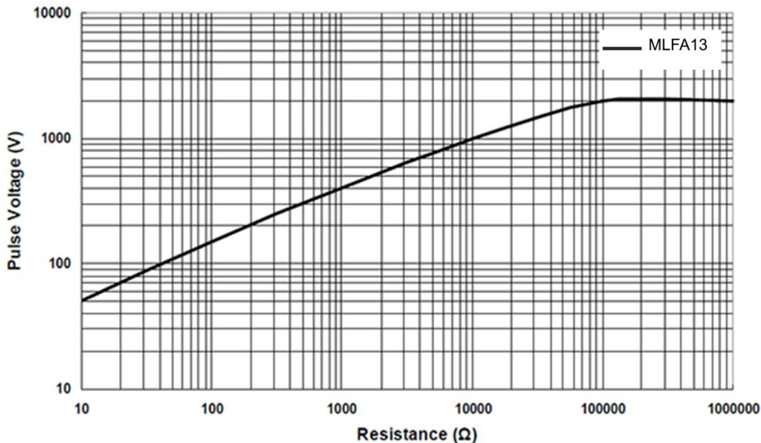
MLFA13 1.2/50µs Lightning Surge
