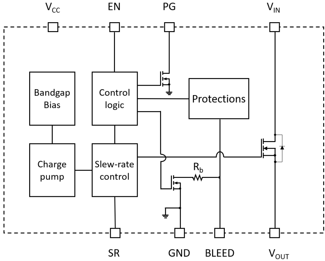
Figure 1. Block diagram
