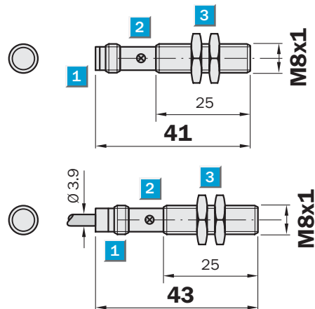
Dimensional drawing
