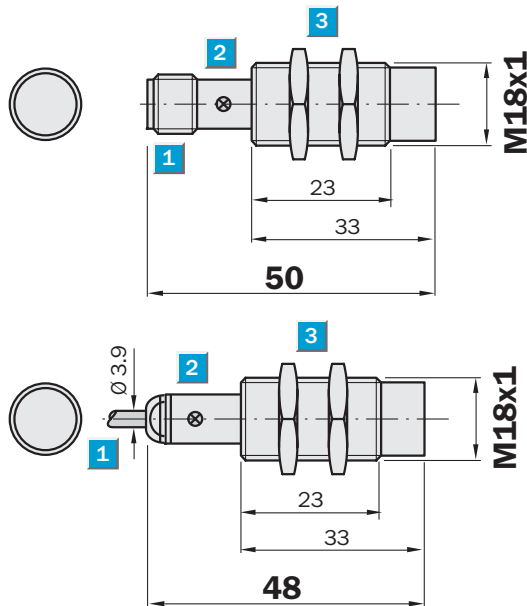
Dimensional drawing
