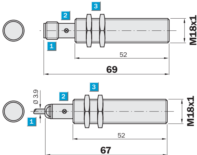
Dimensional drawing
