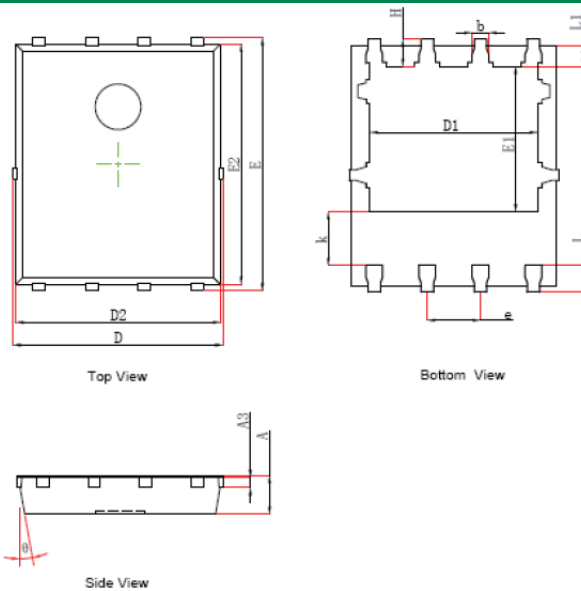
Dimensions-PDFNWB5x6-8L
