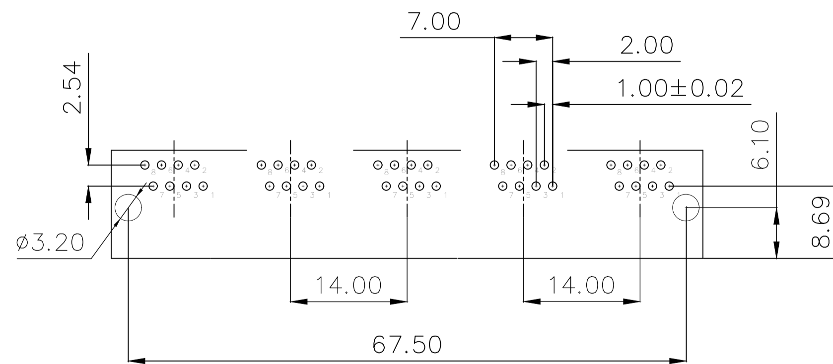
RECOMMENDED PCB LAYOUT TOP VIEW(TOL: \pm 0.05 )
