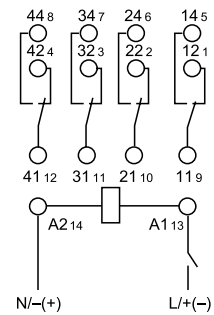
Wiring diagram (without control signal)
