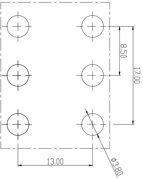
PCB LAYOUT
