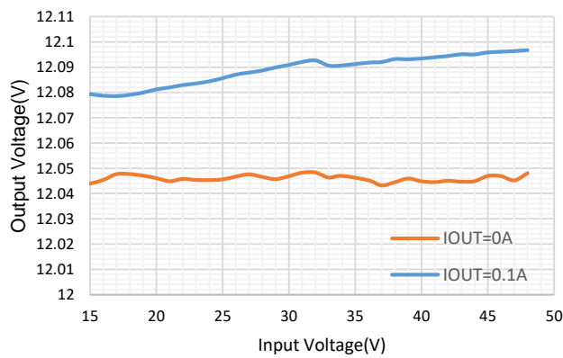
Figure 6. Line Regulation
