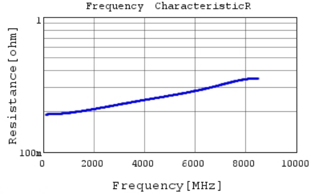
GJM1555C1H2R0BB01 R DCOV, 25degC
