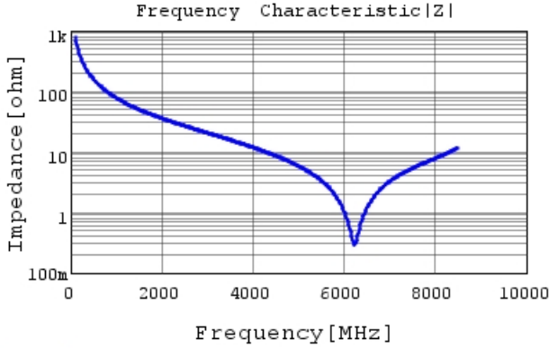
GJM1555C1H2R0BB01 |Z| DCOV, 25degC
