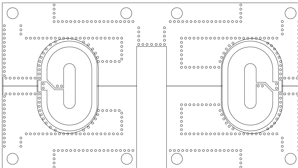
Figure 21. MRF6VP3091NR1(NBR1) 470-860 MHz Broadband 2" x 3.6" Compact Reference Circuit Component Layout — Bottom
