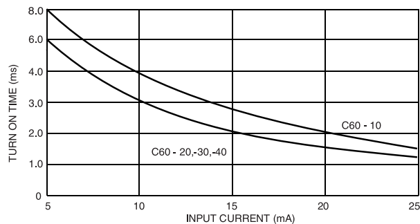
TYPICAL TURN-ON TIME VS. INPUT CURRENT FIGURE 4
