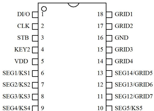
TM1618 SOP-18
