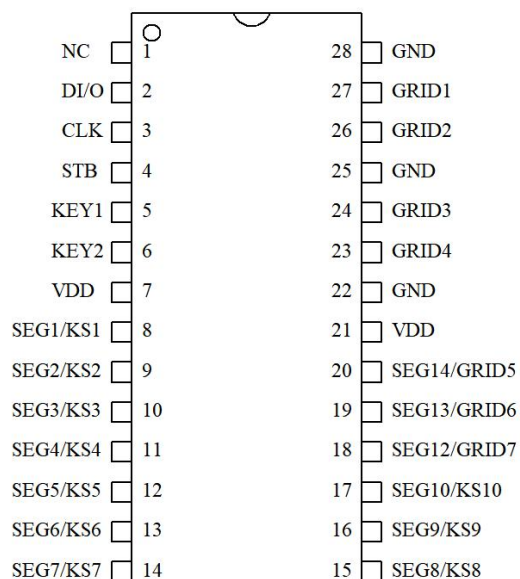
TM1667 SOP-28
