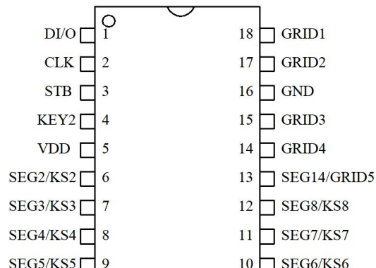
TM1630 DIP-18
