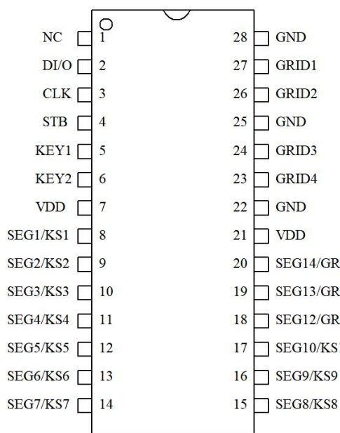
TM1628 SOP/SSOP-28
