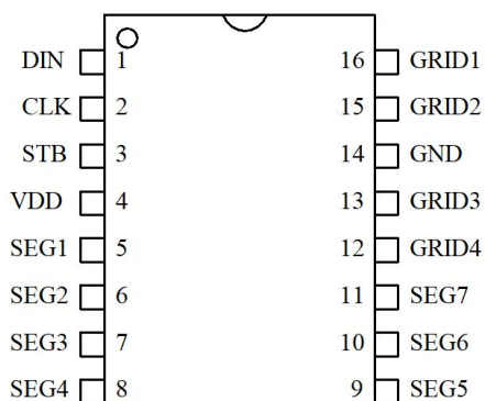
TM1616 SOP-16
