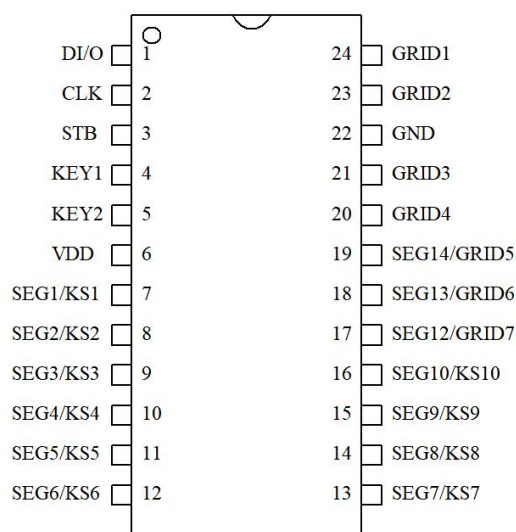
TM1668 SOP/SSOP-24
