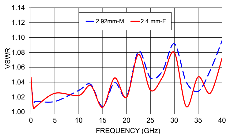
KM-24F+ VSWR
