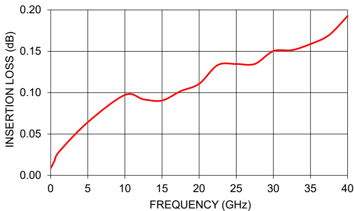
KM-24F+ INSERTION LOSS
