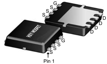
DFN5X6-8L (PDFN-8(5.8x4.9))
