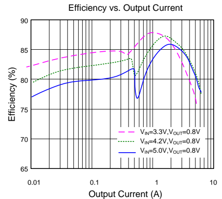
Figure 2. Efficiency
