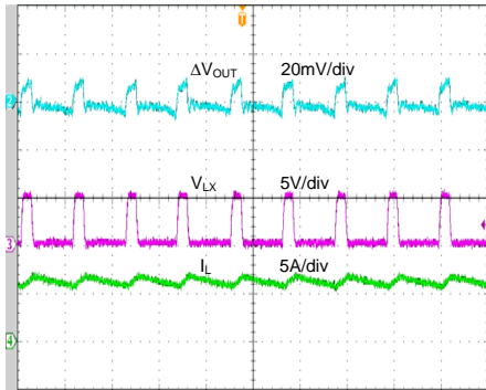
Output Ripple ( V_{IN}=5.0V , V_{OUT}=0.8V , I_{OUT}=6.0A )
