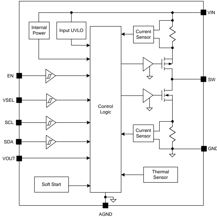
Figure3. Block Diagram
