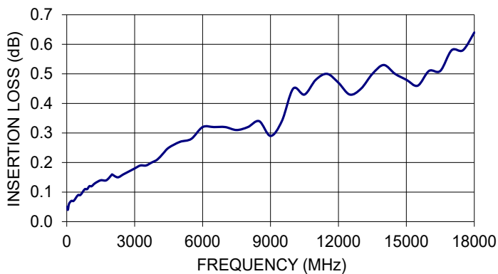
141-8SM+ INSERTION LOSS
