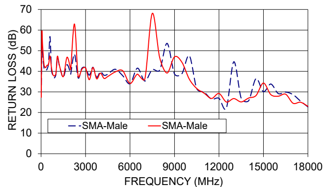
141-8SM+ RETURN LOSS
