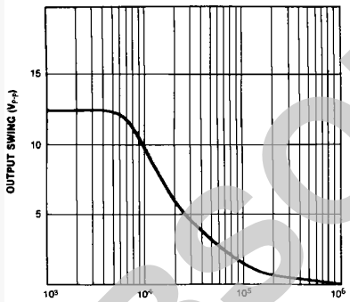
Figure 11. Large Signal Frequency Response
