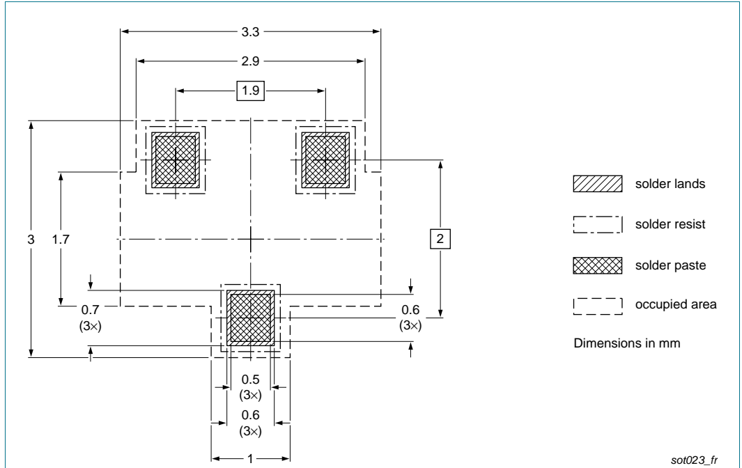
Fig 18. Reflow soldering footprint SOT23 (TO-236AB)
