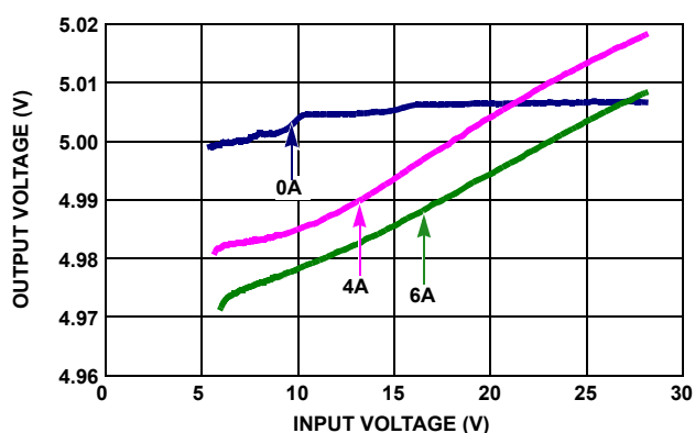
FIGURE 13. OUTPUT VOLTAGE REGULATION vs V_{IN} , CURRENT SHARING, T_A = +25^\circ C , 5V_{OUT} , F_{SW} = 500kHz
