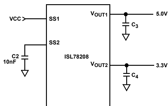
FIGURE 39. INDEPENDENT START-UP
