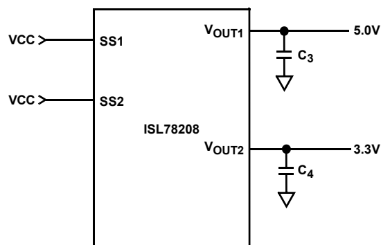
FIGURE 40. RATIOMETRIC START-UP
