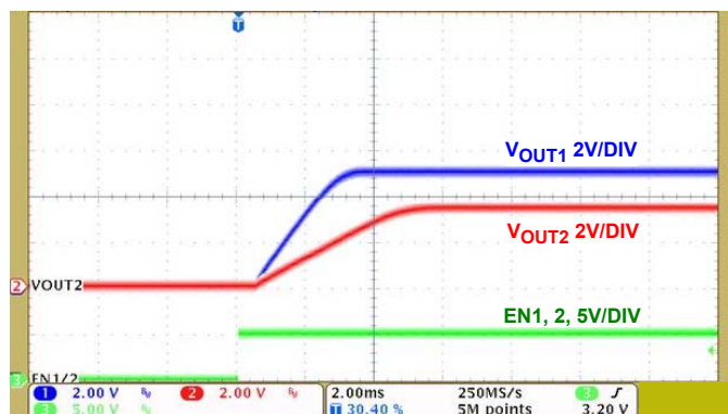
FIGURE 29. INDEPENDENT START-UP SEQUENCING AT NO LOAD
