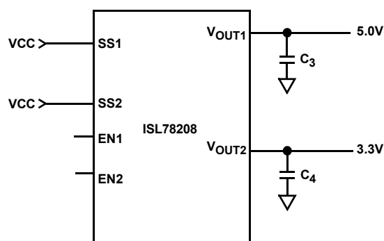
FIGURE 42. OUTPUT SEQUENCING
