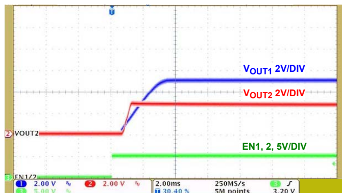
FIGURE 31. ABSOLUTE START-UP SEQUENCING AT NO LOAD
