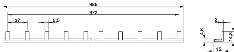
Dimensional drawing
