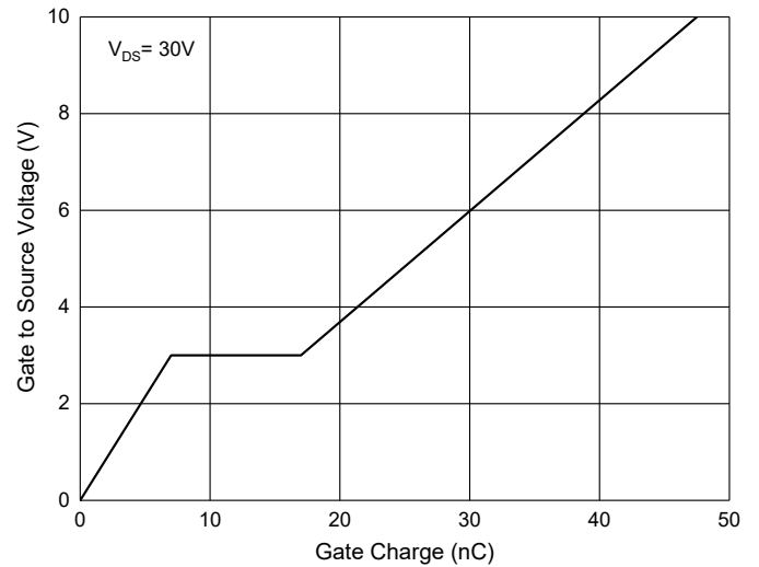
Fig. 4 - Gate Charge
