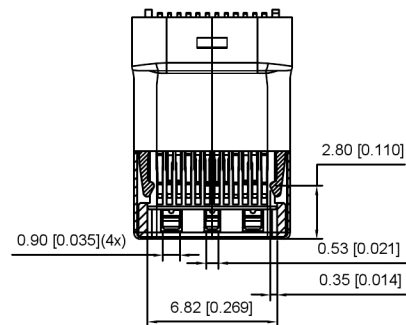
SECT B-B
