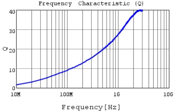
LQP03TN4N3H02 Q
