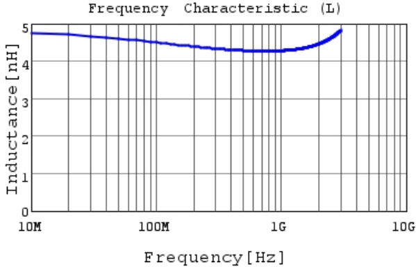
LQP03TN4N3H02 L
